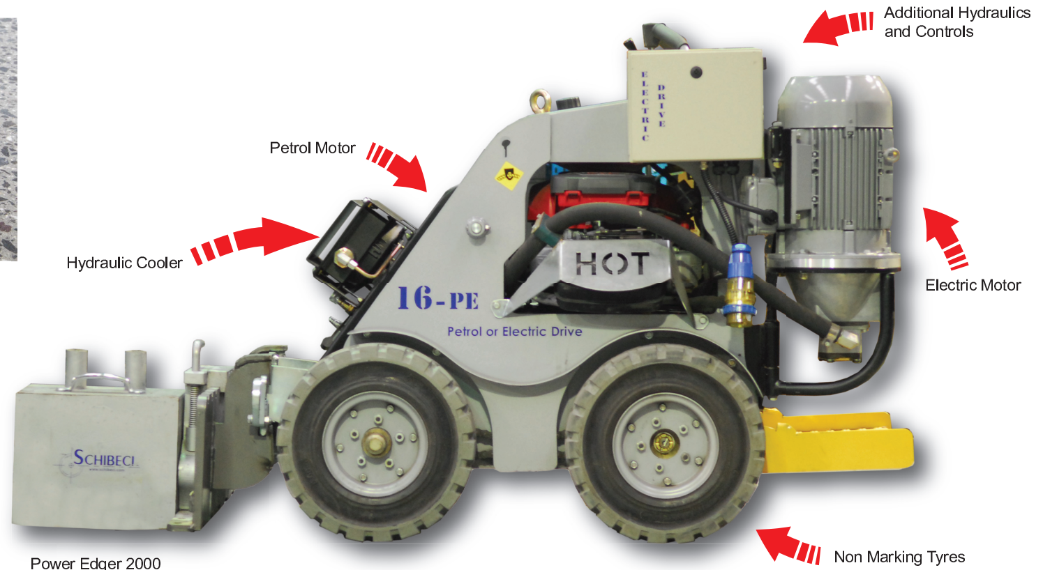
Power Edger 2000 (Milling Mode)
